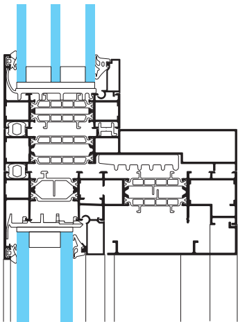
SOLEAL NEXT 75 Add-on mullion with TIGAL pull & slide
