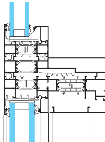
SOLEAL NEXT 65 Add-on mullion with TIGAL pull & slide
