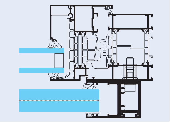
Soleal Next 75: fixation from the outside
