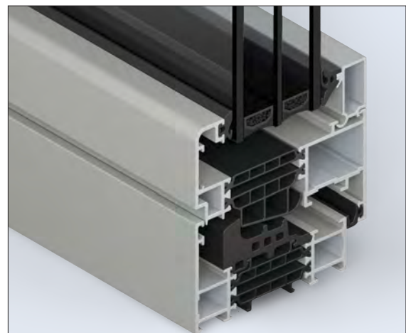
SOLEAL NEXT 75 Visible Standard frame and Soft vent
