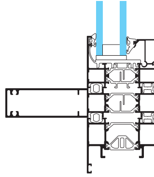
SOLEAL NEXT 65 Reinforced add-on mullion fixe glass and door frame
