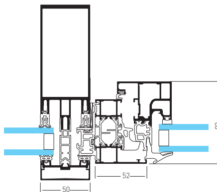
SOLEAL Next 65 Minimal integrated in TENTAL 50
