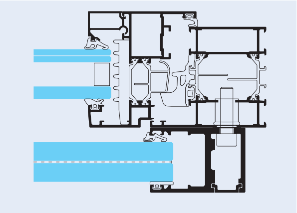
Soleal Next 65: fixation from the outside
