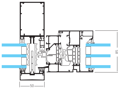
SOLEAL NEXT 75 Visible Flush integrated in TENTAL 50
