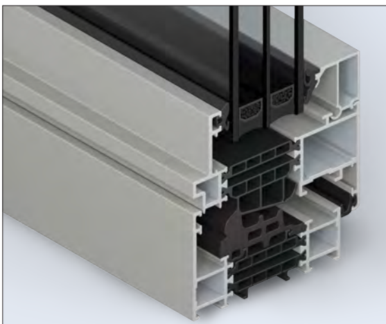
SOLEAL NEXT 75 Visible Standard frame and Step vent
