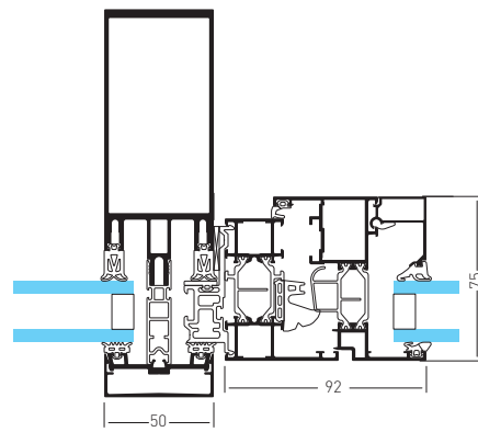
SOLEAL NEXT 65 Visible Flush integrated in TENTAL 50
