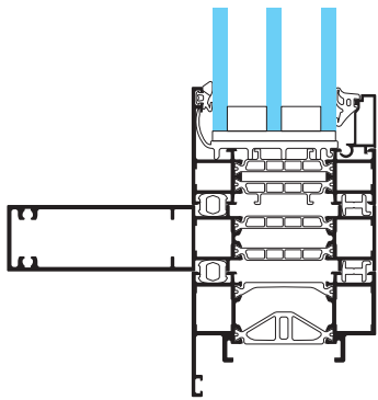
SOLEAL NEXT 75 Reinforced add-on mullion fixe glass and door frame
