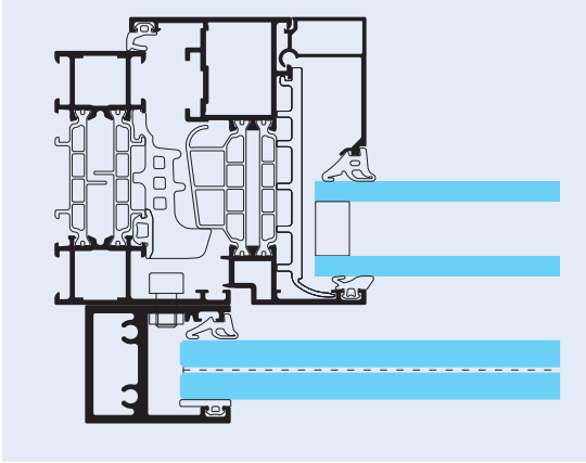
Soleal Next 75: Fixation from the inside
