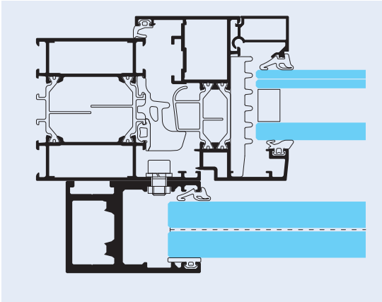
Soleal Next 65: Fixation from the inside
