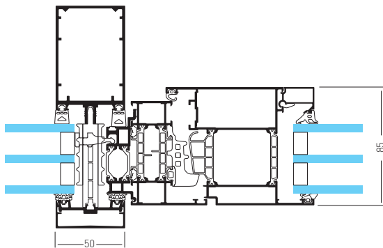
SOLEAL Next 75 Visible Residential Door integrated in TENTAL 50
