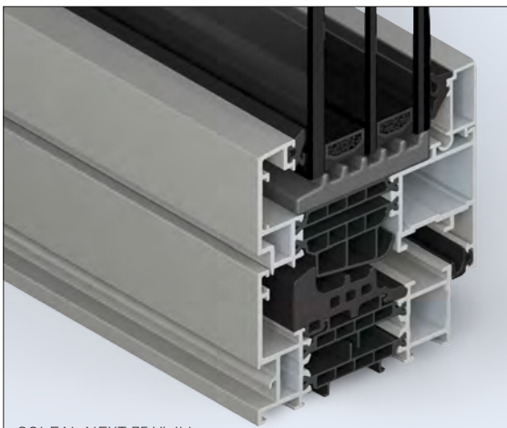
SOLEAL NEXT 75 Visible Concealed drainage frame and Square vent
